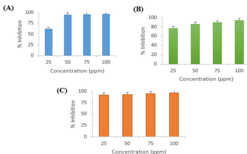
Figure 2. Antioxidant activity of Tetragonula testaceitarsis propolis (P) extract combined with Lepisanthes amoena leaves (K). Combination comparison was showed on (A) P 75% : K 25 %; (B) P50% : K50%; (C) P25%: K75%.
